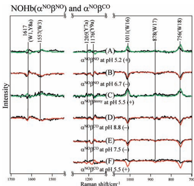
Figure 7. The UVR difference spectra of the liganded forms of Hb against the spectrum (S). \alpha^{\text{NO}}\beta^{\text{NO}} at pH 5.2 in the presence of IHP (A), \alpha^{\text{NO}}\beta^{\text{NO}} at pH 6.7 in the absence of IHP (B), \alpha^{\text{NO}}\beta^{\text{deoxy}} at pH 5.5 in the presence of IHP (C), \alpha^{\text{NO}}\beta^{\text{CO}} at pH 8.8 in the absence of IHP (D), \alpha^{\text{NO}}\beta^{\text{CO}} at pH 7.5 in the absence of IHP (E), and \alpha^{\text{NO}}\beta^{\text{CO}} at pH 5.5 in the presence of IHP (F). (+) or (-) in the figure denotes the presence or absence of IHP, respectively. The 100%T- (Figure 6B) or 100%R-spectrum (Figure 6C) is overlaid with a green or red curve for easy comparison. These spectra were calculated from the corresponding raw spectra shown in Figure SI 2 (A–G) in the Supporting Information.
