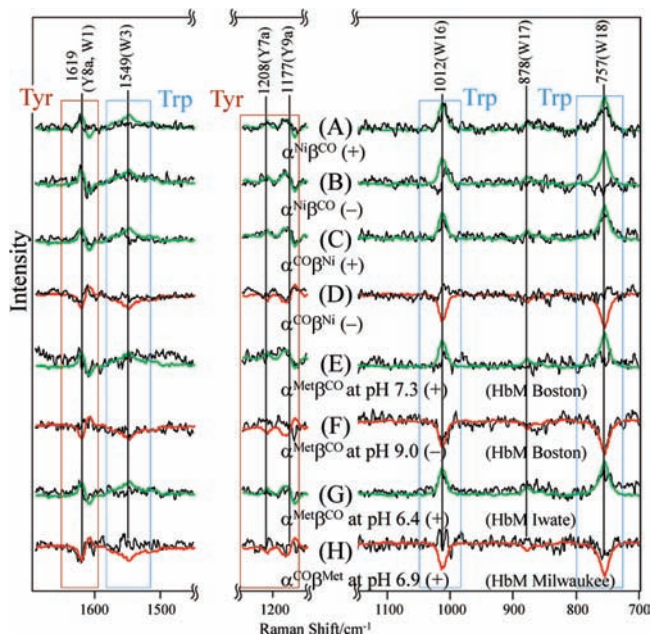
Figure 8. The UVR difference spectra of half-liganded Hbs against the spectrum (S). \alpha^{\text{Ni}}\beta^{\text{CO}} in the presence (A) and absence (B) of IHP and \alpha^{\text{CO}}\beta^{\text{Ni}} in the presence (C) and absence (D) of IHP, HbM Boston \alpha^{\text{Met}}\beta^{\text{CO}} at pH 7.3 in the presence of IHP (E), HbM Boston \alpha^{\text{Met}}\beta^{\text{CO}} at pH 9.0 in the absence of IHP (F), HbM Iwate \alpha^{\text{Met}}\beta^{\text{CO}} at pH 6.4 in the presence of IHP (G), HbM Milwaukee \alpha^{\text{CO}}\beta^{\text{Met}} at pH 6.9 in the presence of IHP (H), and (+) or (-) in the figure denotes the presence or absence of IHP, respectively. Spectra A–D were calculated from the corresponding raw spectra shown in Figure SI 3, and spectra E–H were calculated from the corresponding raw spectra shown in Figure SI 4 in the Supporting Information. See the text for the definition of the spectrum (S) of the \alpha^{\text{Ni}}\beta^{\text{Fe}} and HbMs. The raw spectra of the deoxy forms used for each species are also included in Figures SI 3 and SI 4. The 100%T- or 100%R-spectrum is overlaid with a green or red curve for easy comparison.
